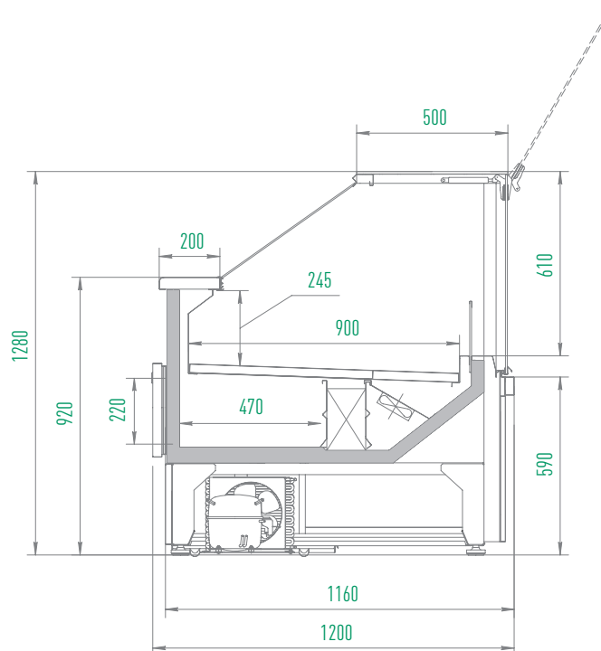
SAMA 125XL/150XL/190XL/250XL LATO / SIDE
